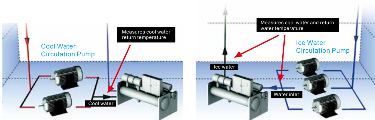
Figure1: Multi-Pump Control
